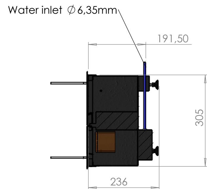
SECTION A-A SCALE 1 : 7.5
